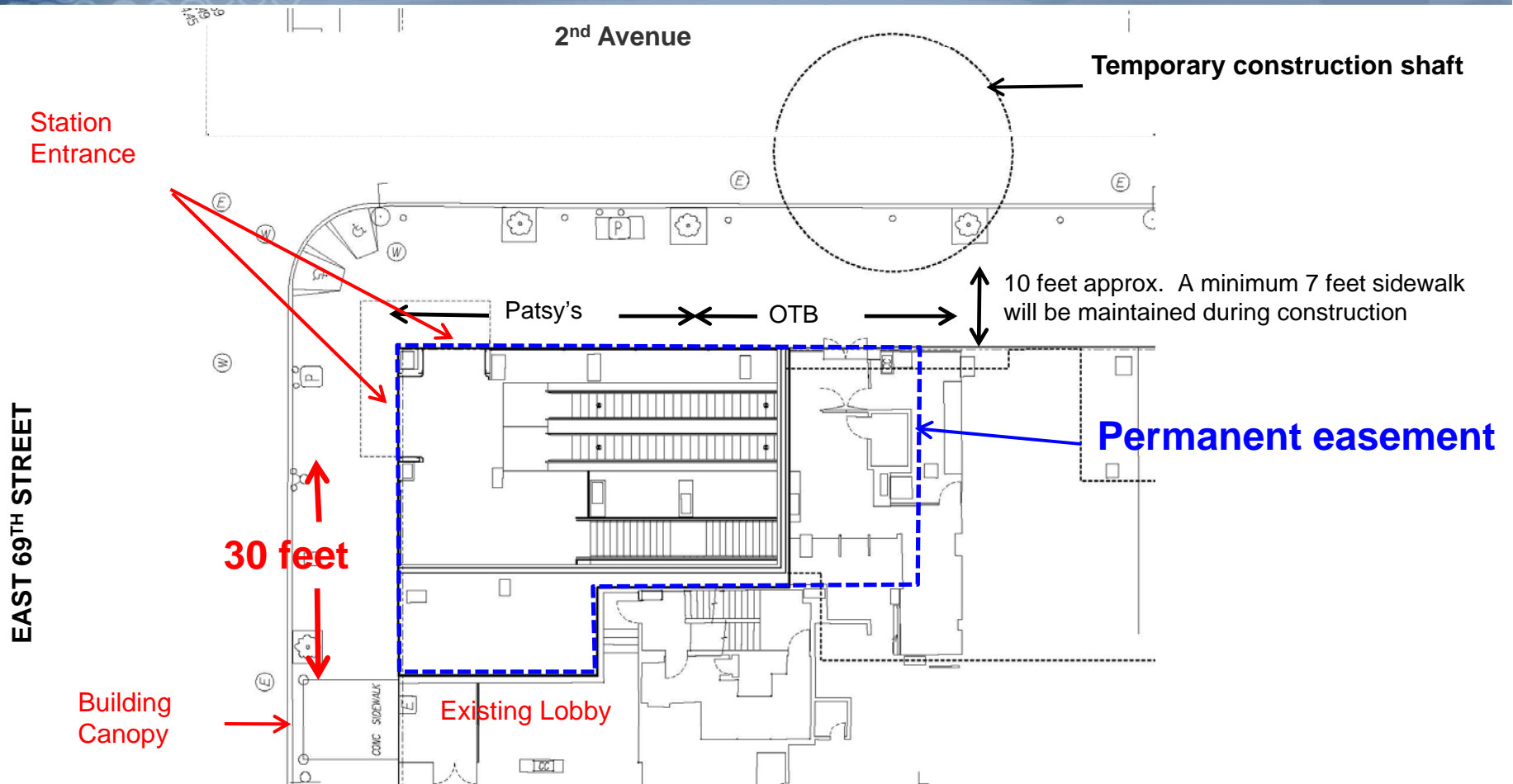
STREET PLAN – PROPOSED
